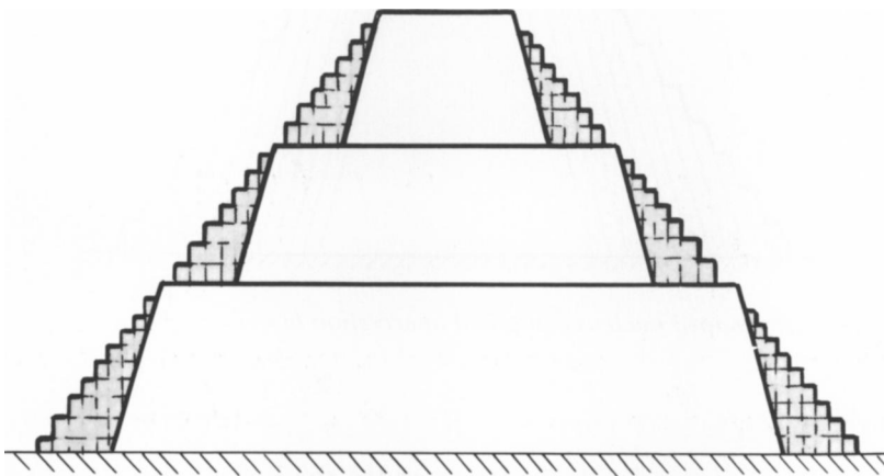
Fig. 19. Stepped structure with external stairways in place.
