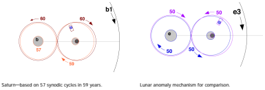
Fig. 34 Proposed mechanisms for the superior planets. The numbers refer to the tooth counts of the gears. All the mechanisms use period relations from Babylonian astronomy. Taking Mars in an example, each superior planet mechanism contains four gears: the fixed input gear G1, the pin gear G2, the slot gear G3 and the output gear G4. The tooth counts of G1 and G2 directly reflect a Babylonian period relation for the planet. The pin gear G2 is mounted epicyclically on a carrier, turning at the rate of the fixed Sun. G2 meshes with G1 and is induced to turn by the rotation of the carrier. G3 is mounted on the opposite carrier on a different axis than G2. The slot on G3 engages with the pin on G2 at distance d from the centre of G2. This induces a variable motion in G4. With an offset of d between the axes of G2 and G3 (where a is the mean distance of the planet from the Sun in AU), this models the synodic phases of the planet. G3 engages with the equally-sized output gear G4, which reverses the output and carries it to the planet's pointer on the Zodiac Dial via a tube. A geometric proof that these mechanisms exactly generate the different and unique models is given at the end of these notes in 4.1. The lunar anomaly mechanism is shown for comparison. The blue gear on the left turns around axis e at the rate of the sidereal Moon, 25419 rotations per year. The gears on the right are mounted epicyclically on eccentric axes on e5 , which turns at the rate of the Line of Apogees of the Moon— 19 \times 532(17 \times 2.23) rotations per year. The tooth counts of the first two gears in the system, G1 and G2, exactly reflect the assumed planetary period relation. The tooth counts of the last two gears have no special meaning: they are simply chosen so that two equal gears with much the same module fill the space between the central axis and the axis of the gear with the slot. First, we look in detail at a practical embodiment of these ideas for the planet Mars, then we build all the superior planets onto the SPP in our new model.
