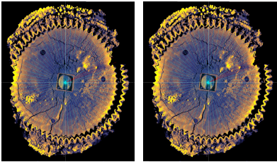
Fig. 33 X-ray CT section of gear in Fragment D. The X-rays have a false-colour scale to enhance the tooth tips for counting. Two alternative counts are shown in red for 63 teeth (on the left) and 64 teeth (on the right).
