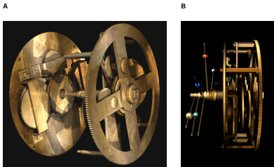
Fig. 38 Computer model of The Planet Module
