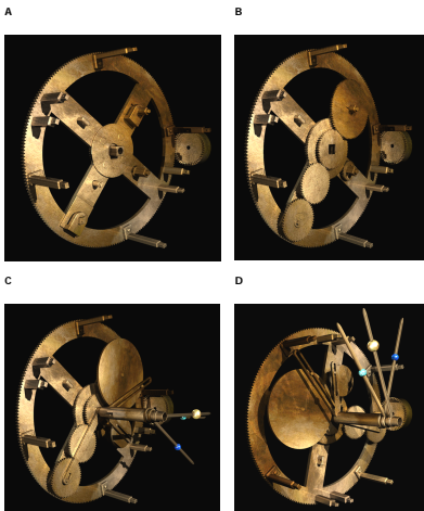
Fig. 30 Computer model of Solar Anomaly & Inferior Planets & Mechanisms on b1 (A) b1 with the bearings and arbors for the solar anomaly and inferior planets. (B) The gears for the solar anomaly and inferior planet mechanisms with Venus on the 1 o'clock spoke, Mercury on the 4 o'clock spoke and the Sun on the 10 o'clock spoke. (C) The solar and inferior planet mechanisms. (D) The solar and inferior planet mechanisms, b1 has been rotated so that Mercury is at 1 o'clock, the Sun at 4 o'clock, and Venus at 10 o'clock.
