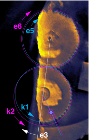
Fig. 8 Diagram of the lunar anomaly mechanism (from Freeth et al. 2006, 590). The diagram is superimposed on a false-colour X-ray CT slice through Fragment A.
