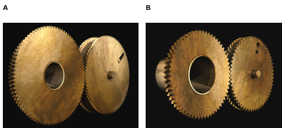
Fig. 36 Computer Reconstructions of Jupiter and Saturn mechanisms (A) Jupiter Mechanism based on the period relation (76, -83). (B) Saturn mechanism based on the period relation (57, -59).
