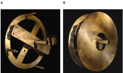
Fig. 29 Computer reconstruction of b1 with plates carried by the pillars. (A) The Main Plate is attached to the short pillars. The input crown gear can be seen on the right. (B) The Superior Planet Plate (SPR) is attached to the long pillars. Our proposal is that a mechanism for the solar anomaly and mechanisms for all five planets were contained within the space in front of the Main Drive Wheel, b1. In our model, mechanisms for the solar anomaly and the inferior planets are attached to the spokes of b1; and mechanisms for the superior planets are attached to the rear side of the circular plate carried by the support pillars. To enable our model to work this circular plate
