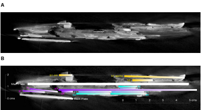
Fig. 7 X-ray CT showing cross-section of gearing in Fragment A (A) The gears are hard to identify in cross-section. (B) The gears are identified in the same colours as Fig. 6.
