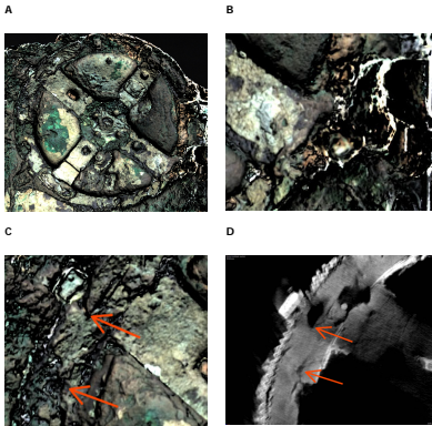
Fig. 22 Short pillar attachments on the Main Drive Wheel (A) The Main Drive Wheel, showing the pillars on the right-hand side. (B) Front view of the two short pillars. (C) The symmetrically opposite position on the Main Drive Wheel. (D) The X-ray CT shows holes in these positions, which suggest that rivets might originally have been there. The short pillars are riveted directly to b1, rather than attached with brackets. In the symmetrical position on the opposite side of b1, possible rivet holes can be seen in the X-ray CT. In our model, we reconstruct four short pillars consisting of two pairs on opposite sides of the Main Drive Wheel. Why these pillars are offset from a symmetrical position relative to the spokes is not clear, though it may be designed so that their rivets avoid the dovetail joints, which attach the spokes to the rest of the wheel. Like the long pillars, the short pillars also appear to be designed to carry a plate.
