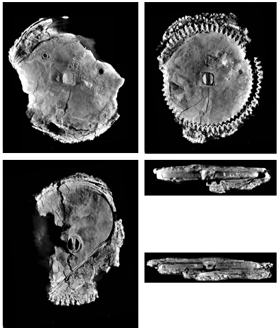
Fig. 32 X-ray CT of Fragment D. Three parallel slices through Fragment D. The 1 st and 2 nd slice are 2 mm apart and the 2 nd and 3 rd 1.5 mm apart. Two orthogonal slices through the hub of the gear.
